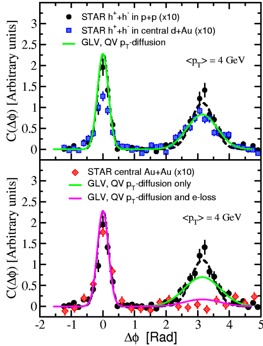
Fig. 14. Azimuthal correlations of high- p_T hadrons for d+Au collisions (squares, top plot) and central Au+Au collisions (diamonds, bottom ), in comparison to data from p+p collisions (circles). The data are compared to a model calculation in the GLV formalism. Black dashed lines are a Gaussian fit to the correlation function
