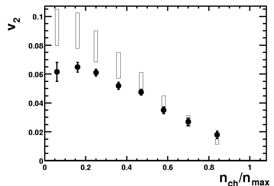
Fig. 6. Elliptic flow parameter v_2 for Au+Au collisions at 130 GeV as a function of collision centrality (STAR)
