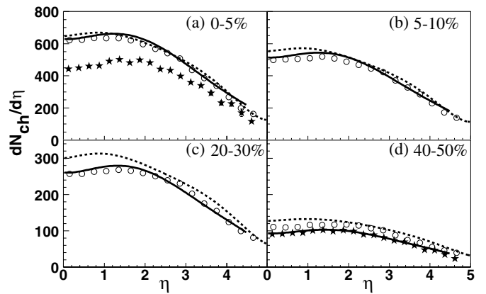
Fig. 4. Charged particle pseudo-rapidity distributions from BRAHMS for Au+Au collisions in four bins of centrality, in comparison to saturation model calculations ( solid line ), the AMPT model ( dashed line ) and data from p+p collisions scaled by the mean number of participant nucleon pairs (stars)
