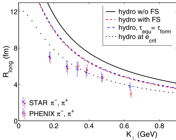
Fig. 16. R_{long} , the coherence length measured in longitudinal direction measured by two-pion Bose-Einstein correlations, as a function of pair transverse momentum k_{\perp} . Hydrodynamic model calculations are shown in comparison to data from STAR and PHENIX
