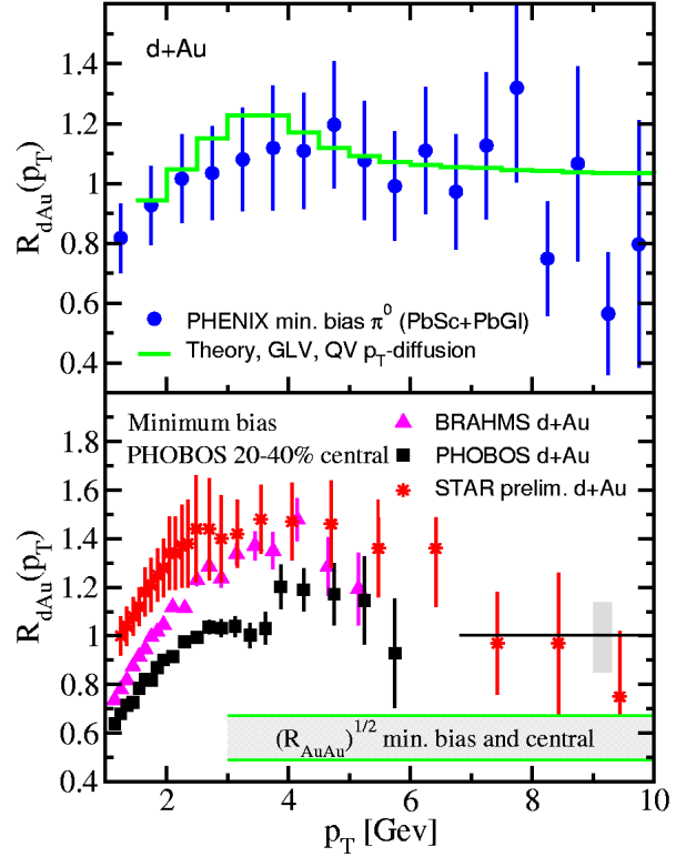
Fig. 13. Nuclear modification factor R_{dAu} as a function of p_T for d+Au collisions at \sqrt{s} = 200 GeV. Data are shown for neutral pions (top) and charged hadrons (bottom). The \pi^0 data are compared to a model calculation in the GLV formalism
